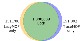
Fig. 13. Venn diagram for no. of unique traces found by LAZYMOP only, TRACEMOP only, and both.
