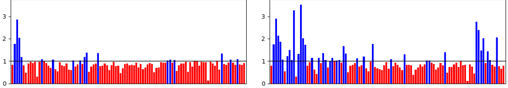
Fig. 9. Number of times faster (blue) or slower (red): LAZYMOP vs. JAVAMOP (left); LAZYMOP e vs. JAVAMOP (right).
